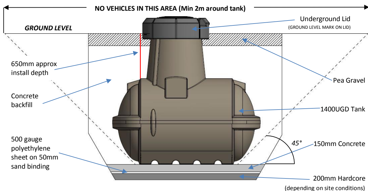
Figure 2: Underground Fuel Tank Installation Image
