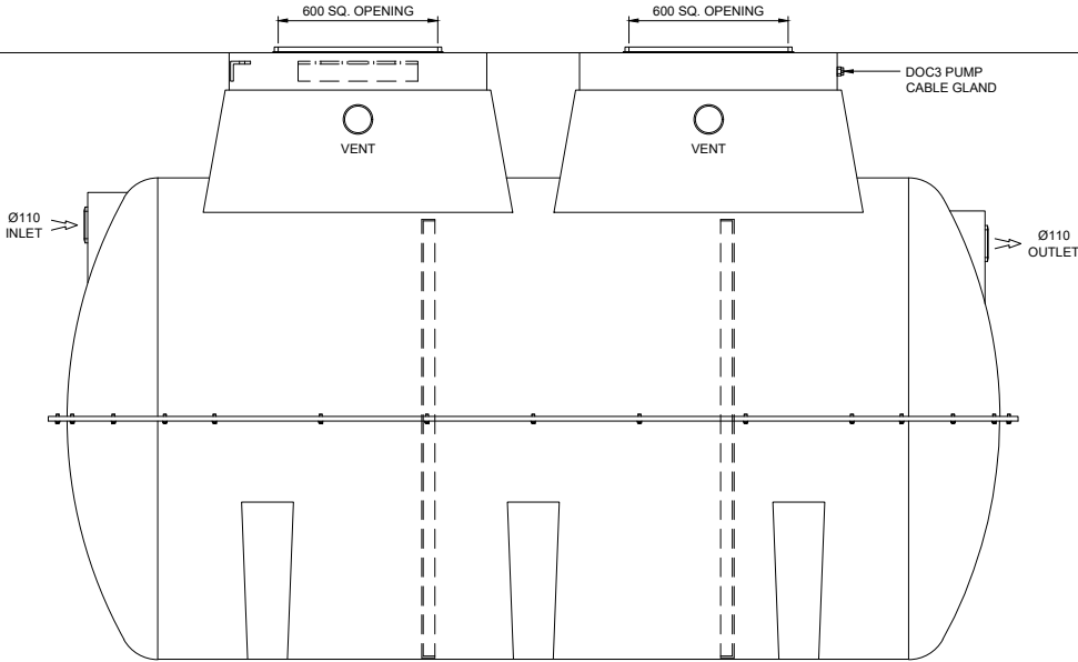
SIDE ELEVATION
