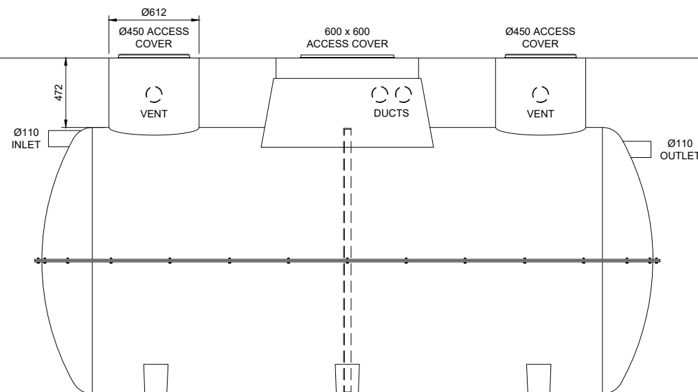
SIDE ELEVATION
