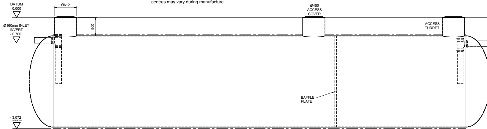
SIDE ELEVATION
