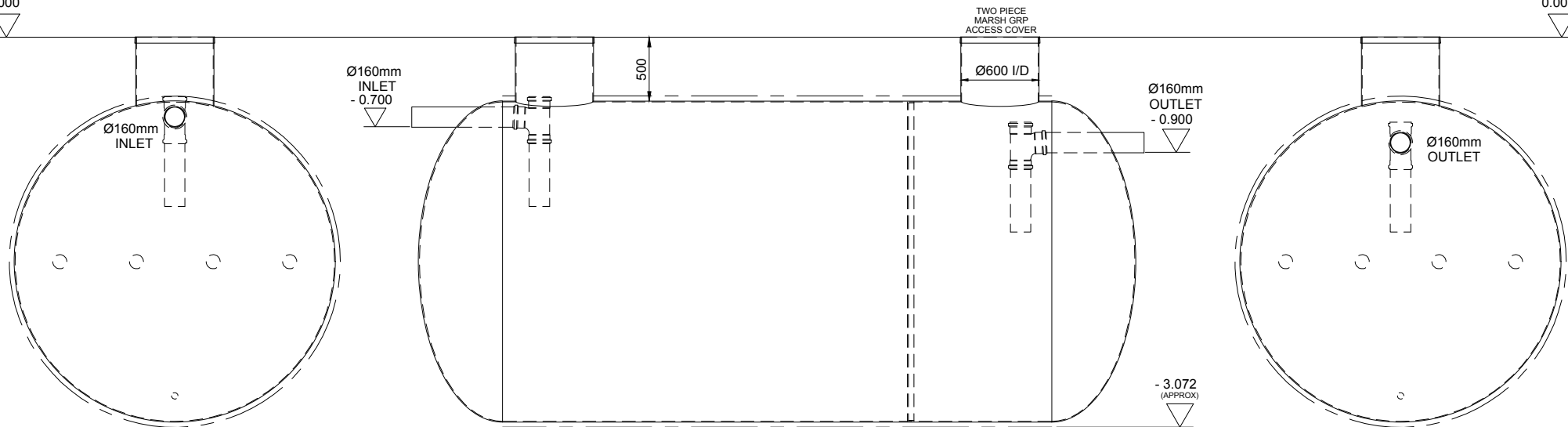
SIDE ELEVATION
