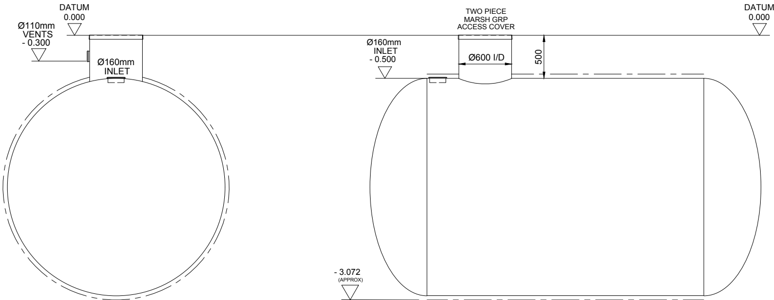
VIEW ON INLET
