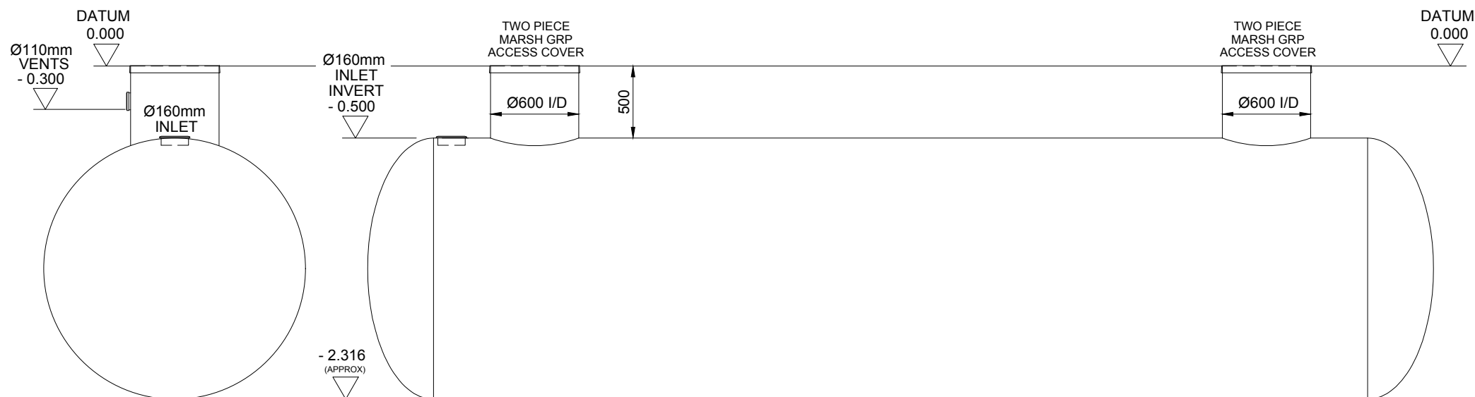
SIDE ELEVATION
