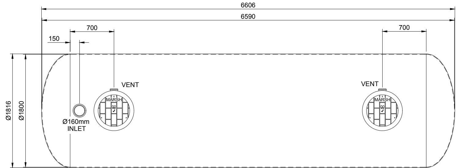
PLAN
