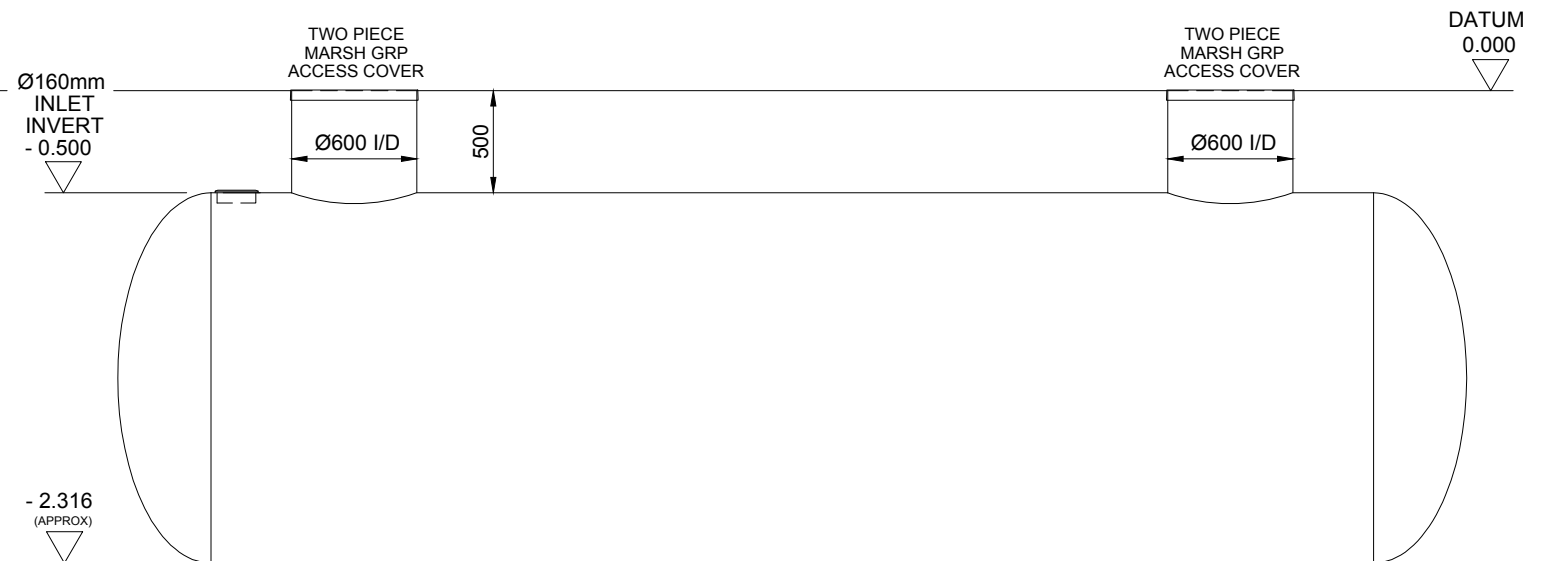
SIDE ELEVATION
