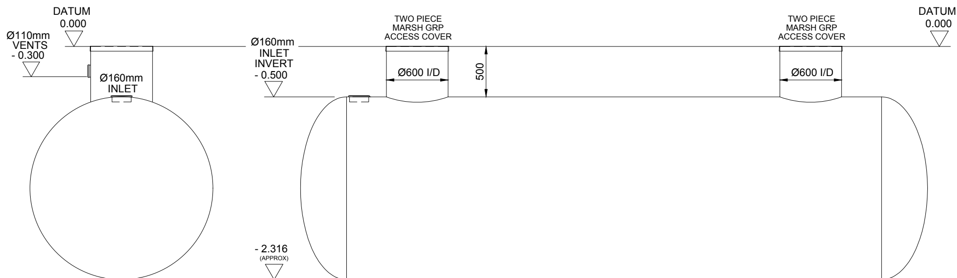
SIDE ELEVATION
