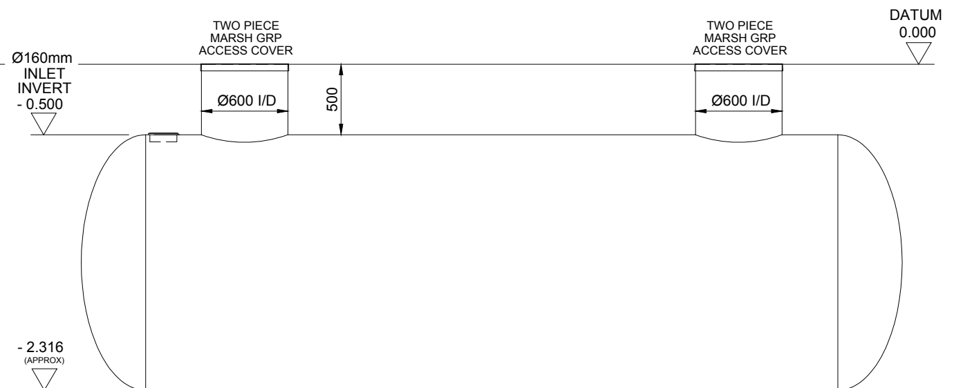
SIDE ELEVATION
