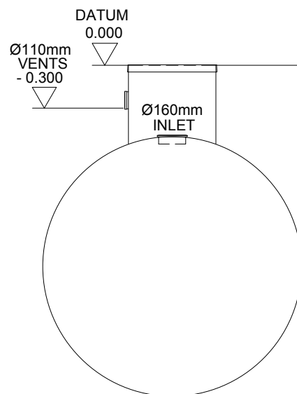
VIEW ON INLET END
