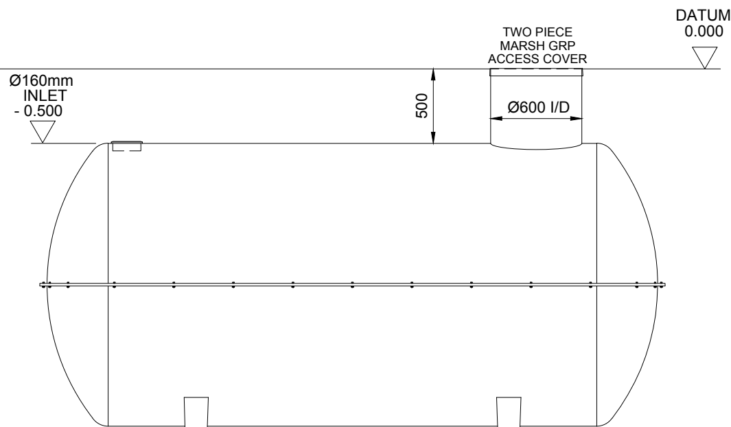
SIDE ELEVATION
