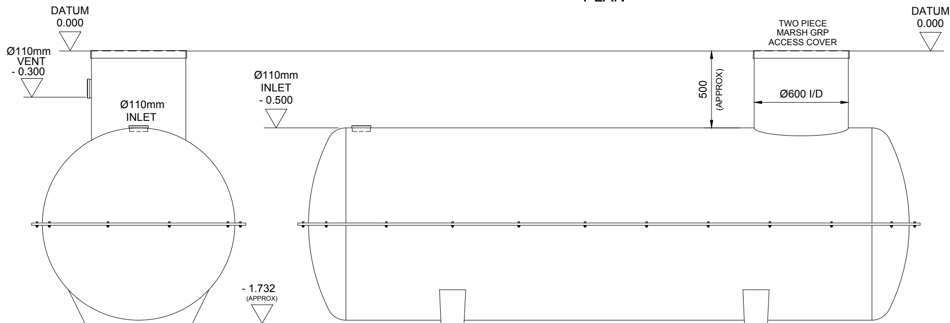
VIEW ON INLET
