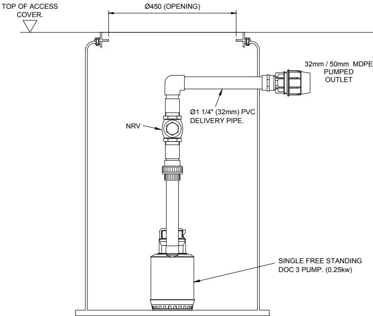
SECTION THRO' TANK
