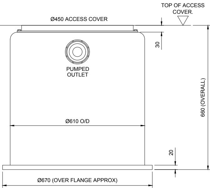
VIEW ON OUTLET
