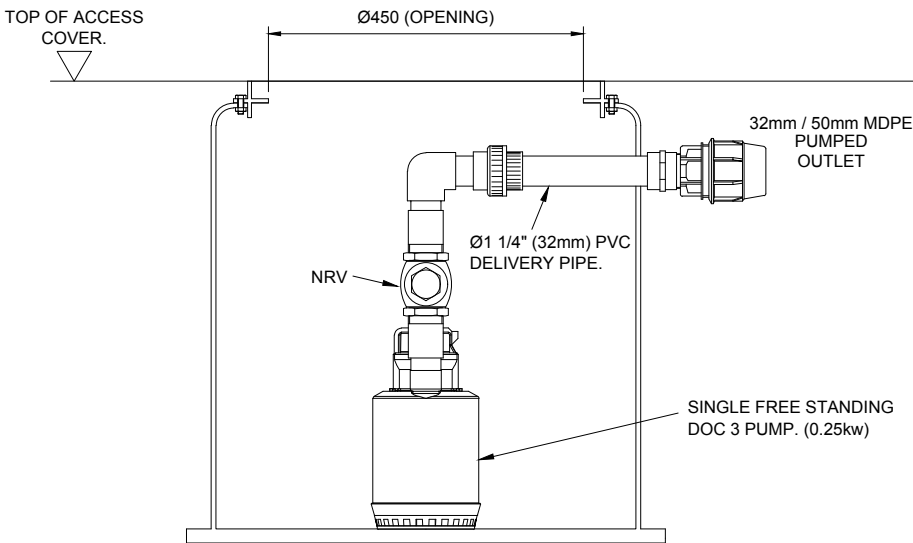
SECTION THRO' TANK
