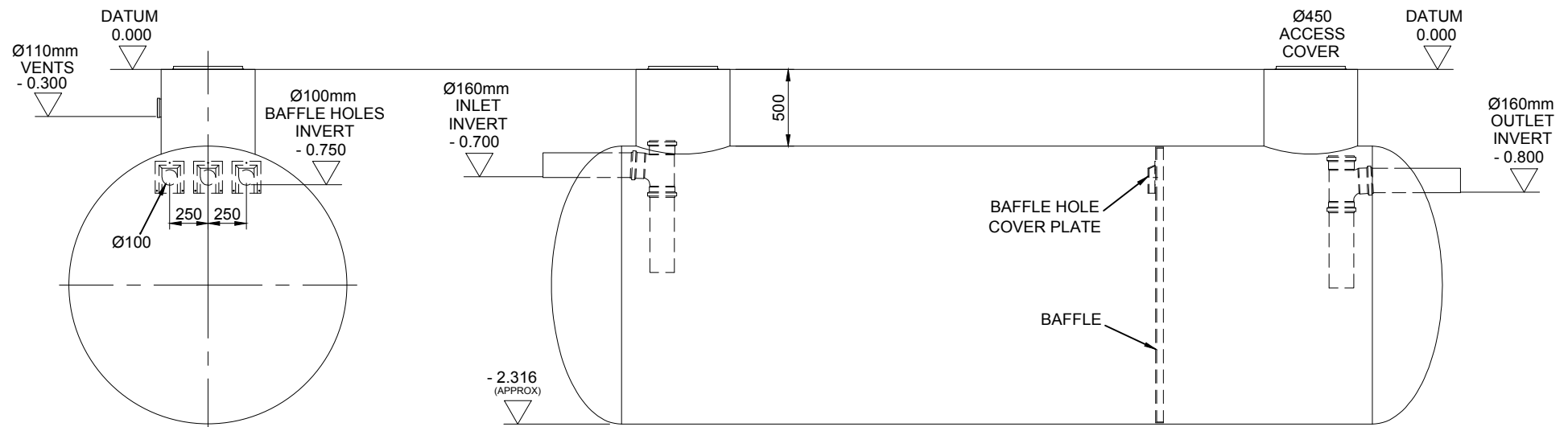
SIDE ELEVATION
