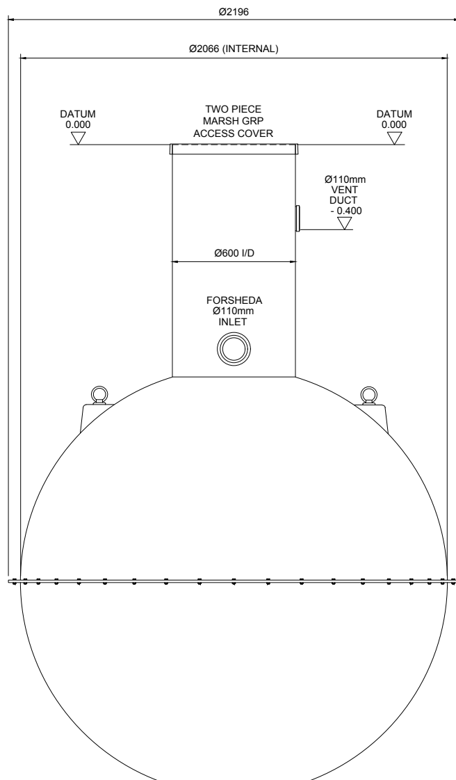
VIEW ON INLET
