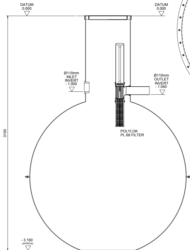
SECTION THRO' TANK
