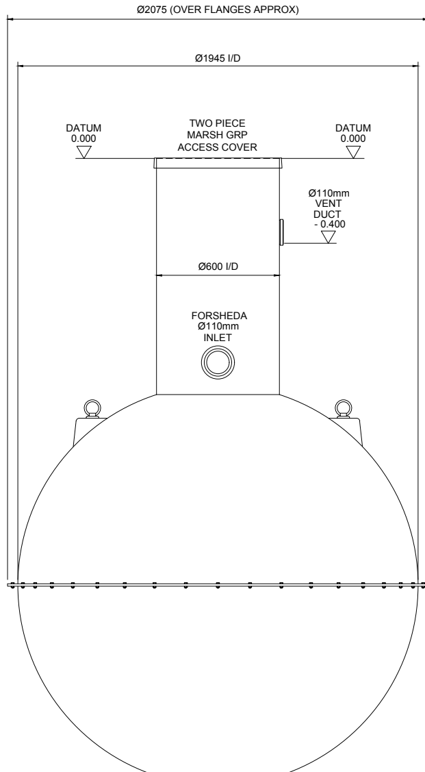
VIEW ON INLET
