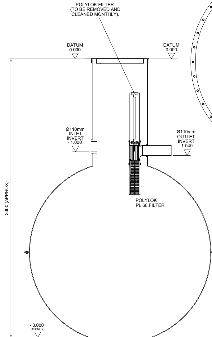
SECTION THRO' TANK
