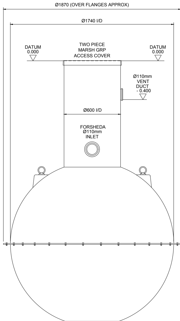
VIEW ON INLET
