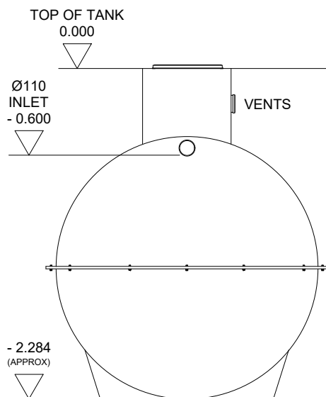
PLAN 600 x 600 ACCESS COVER VENT VENT VENT Ø110 INLET Ø110 OUTLET
