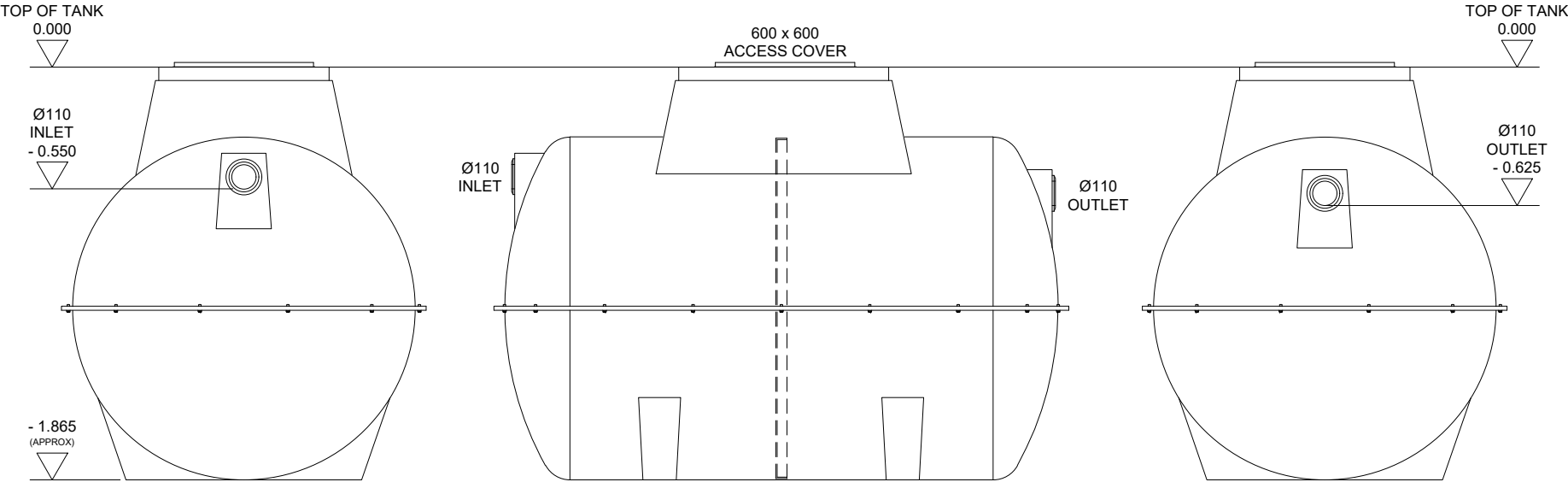
VIEW ON INLET
