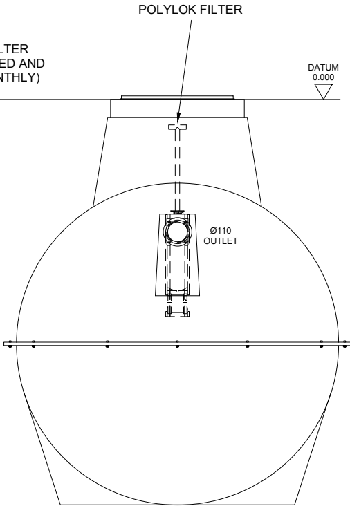
VIEW ON OUTLET
