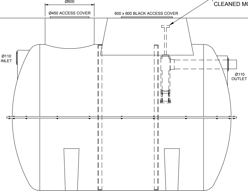
SIDE ELEVATION
