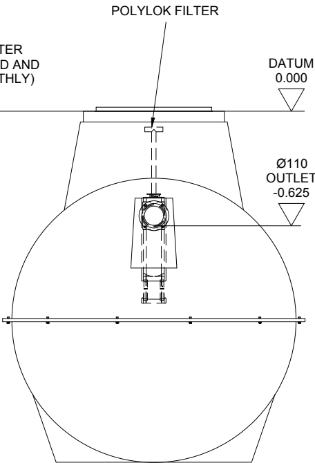
VIEW ON OUTLET
