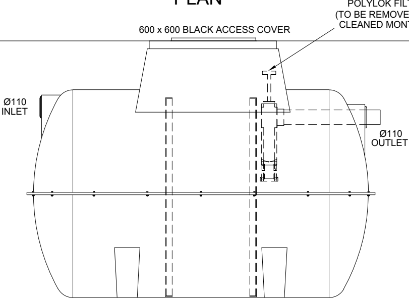
SIDE ELEVATION
