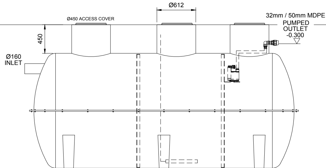
SIDE ELEVATION
