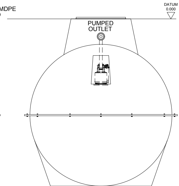
VIEW ON OUTLET
