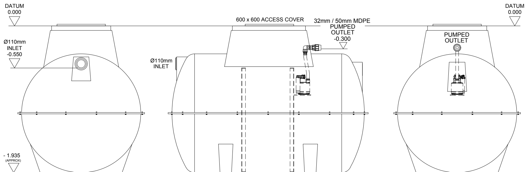
VIEW ON INLET
