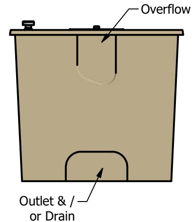
View C
