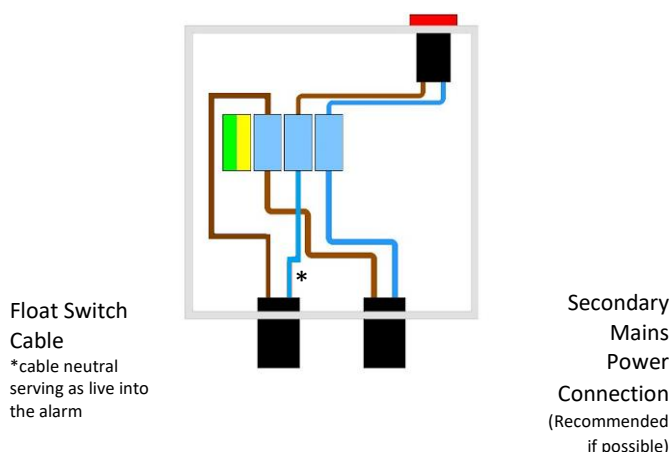
Figure 18: Wiring for Single Channel Alarm Box
