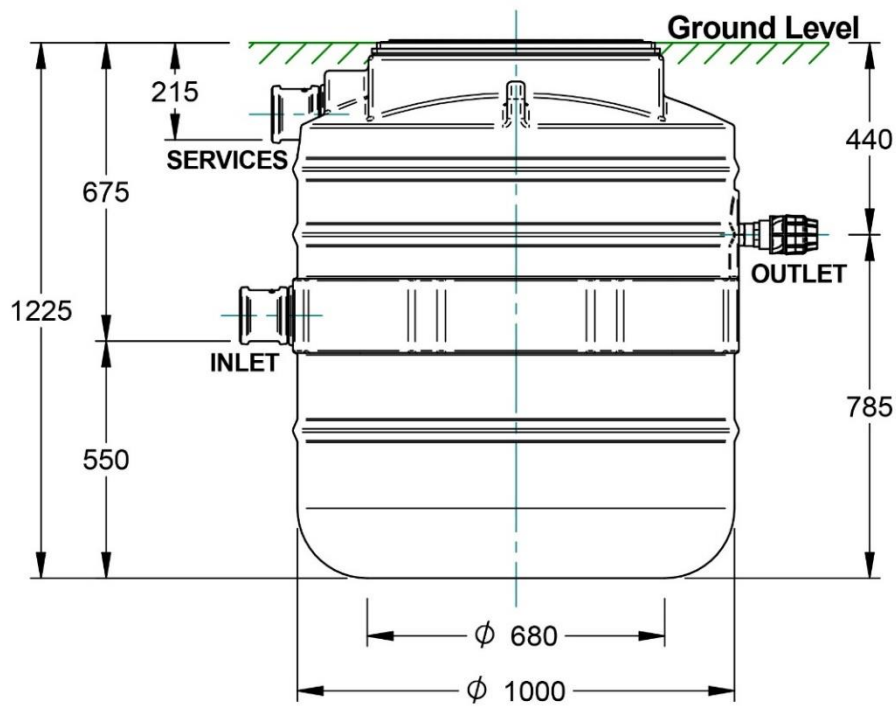
Figure 8: 800LT Pump Station dimensions
