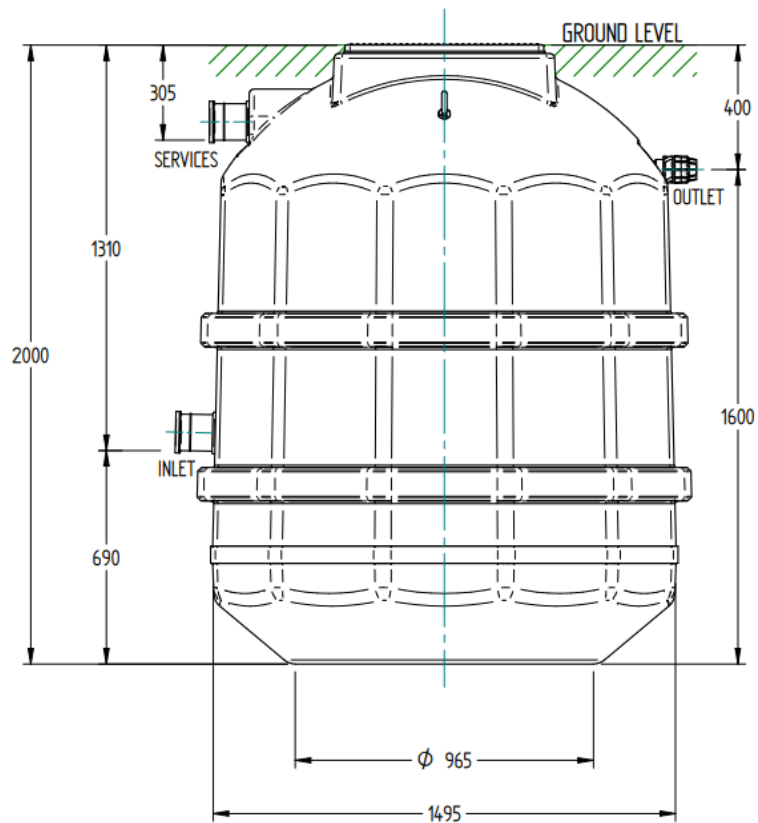
Figure 11: 2700LT Pump Station dimensions
