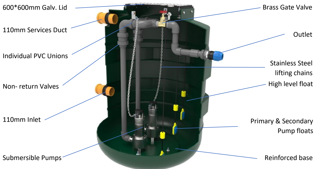
Figure 15: 1100LT Twin Pump Station (Model 1100PSV2)
