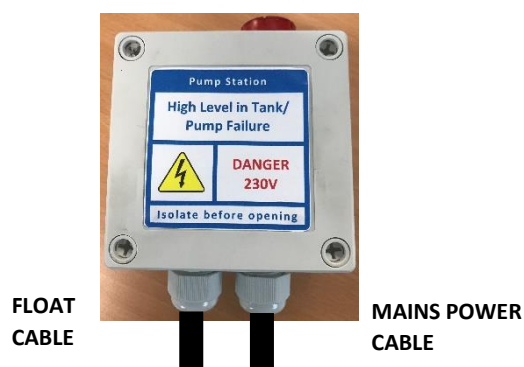
Figure 17: High level Alarm box used in pump stations
