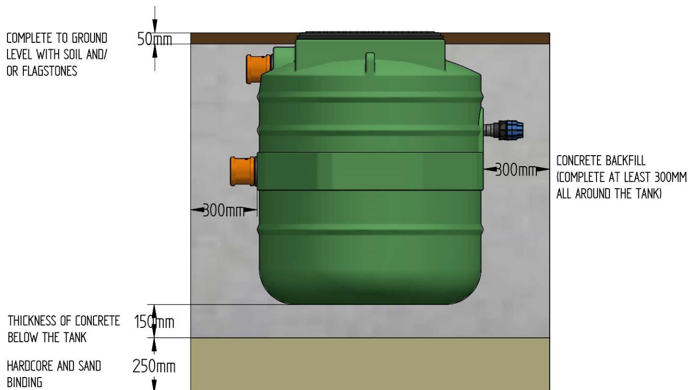
Figure 13: Typical Pump Station Concrete Backfill Installation
