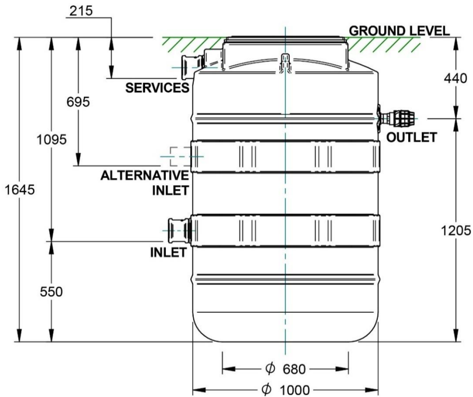
Figure 9: 1100LT Pump Station dimensions
