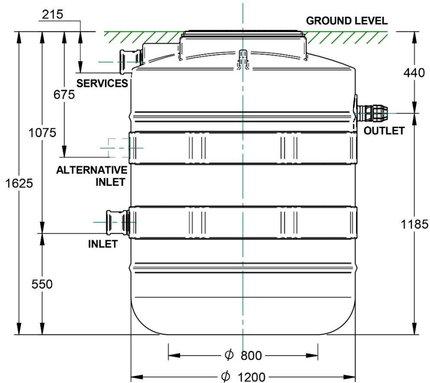
Figure 10: 1550LT Pump Station dimensions
