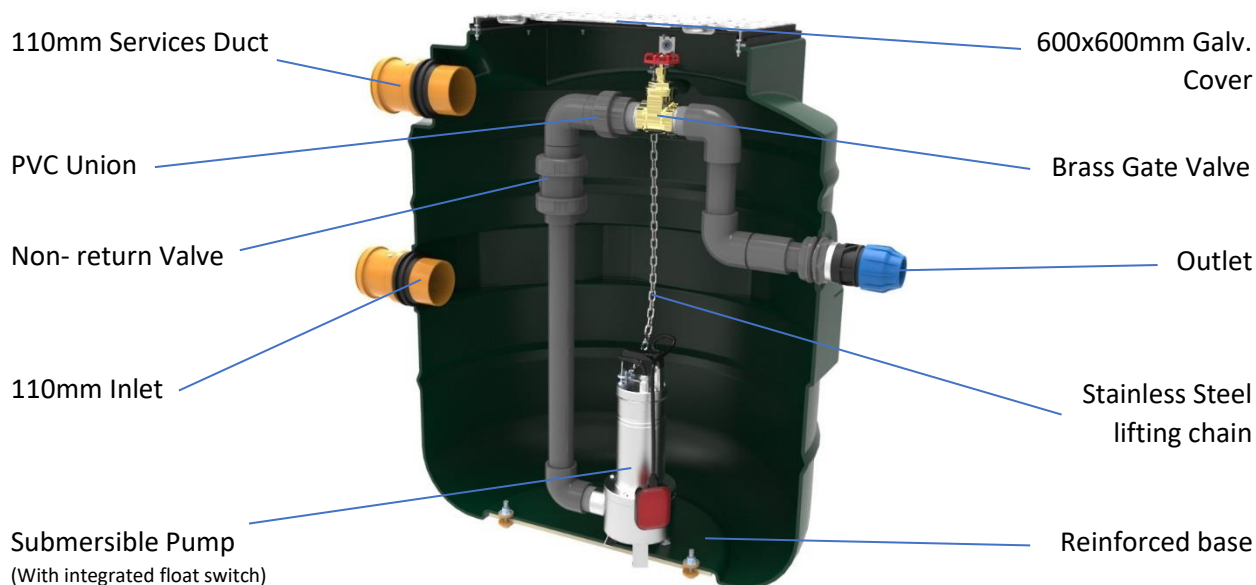
Figure 14: 800LT Pump Station (Model 800PSV1)
